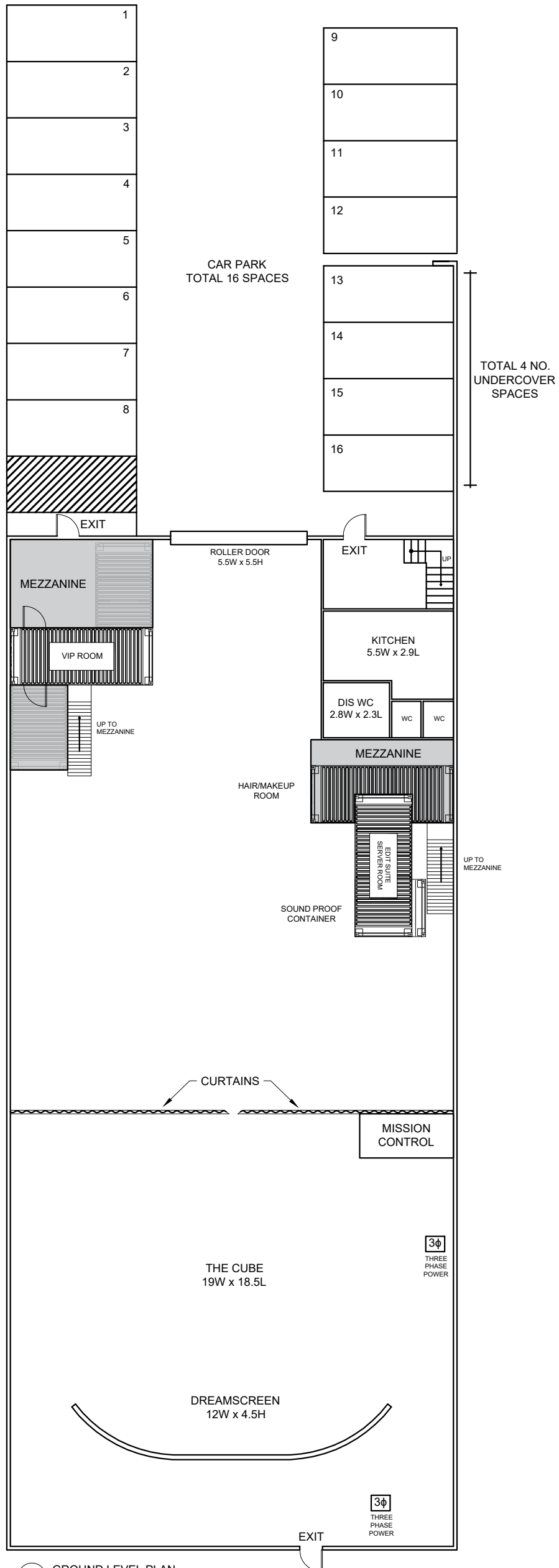
1 GROUND LEVEL PLAN
